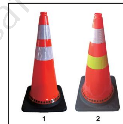
LZ005 SOFT PVC TRAFFIC CONE Height:75cm Weight:2.3kgs/2.5kgs Base size:37*37cm Tape:10cm+10cm 12cm+12cm or as requested 150pcs/M 3 5000pcs/20"
