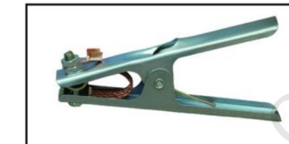
ET008(300A) JAPANESE TYPE EARTH CLAMP 100PCS/CTN 64X43X19CM
